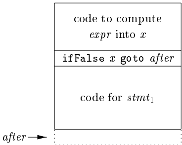
Figure 2.42: Code layout for if-statements
