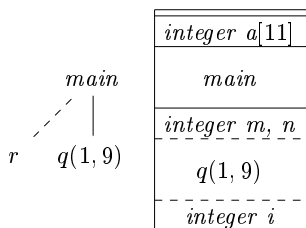
(a) Frame for main
